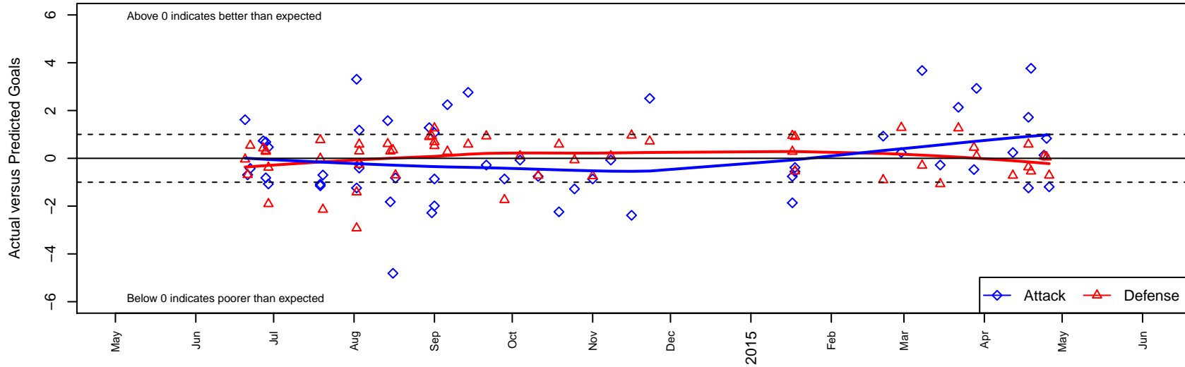
WPFC Fury Black G00 Dots are actual minus expected GF (blue circles) and GA (red triangles). Blue line is smoothed change in attack strength. Red is smoothed change in defense strength.
